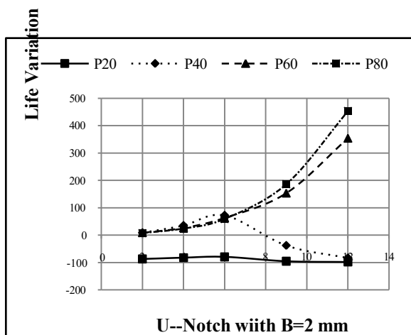
Fig 13: Variation of Percentage Error of Life with U- Notch Radius B = 2 for Different Position from Root of the Blade.
