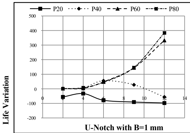
Fig 12: Variation of Percentage Error of Life with U- Notch Radius B = 1 for Different Position from Root of the Blade.
